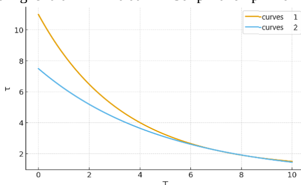
Fig. 11. Typical nature of changes in the hydraulic density of plunger pairs under normal operating conditions: 1 – with single-stage filtration; 2 – with two-stage filtration speed of 30 \text{ km/h} , which corresponds to 8730 hours
