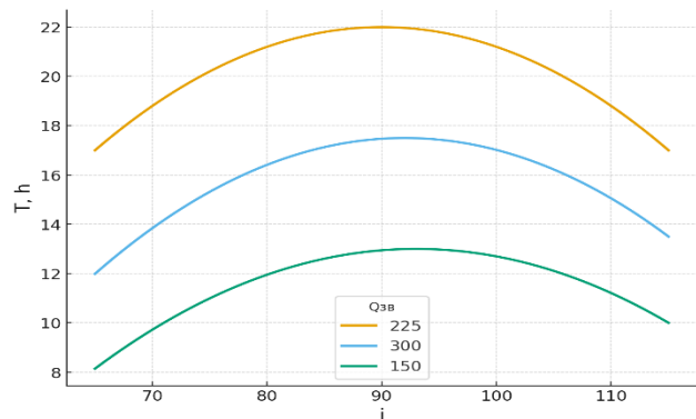
Fig. 6. The influence of the quality i of the corrugations on the service life of the T element before servicing at different air flow rates by the engine Q_{eng}(\gamma_1=0,5 g/m^3; \Delta h_{pr}=700 mm H_2O)
