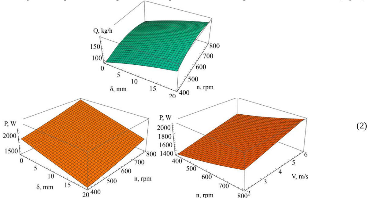
Fig. 3. Dependence of the productivity Q and power consumption P of the developed castor seed cleaning machine on the distance between the concave and crushing cones \delta and the rotation speed of the crushing cone n
