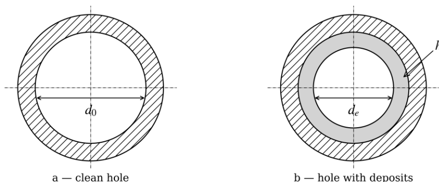
Fig. 2. Calculation model of a hole in the 6A1-20c2-50 nozzle:
