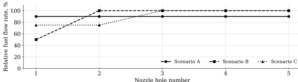
Fig. 3. Calculated distribution of relative fuel flow rates among nozzle holes for Scenarios A, B and C in Table 3
