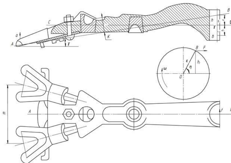
Fig. 2. Lever of the first type of clipper
