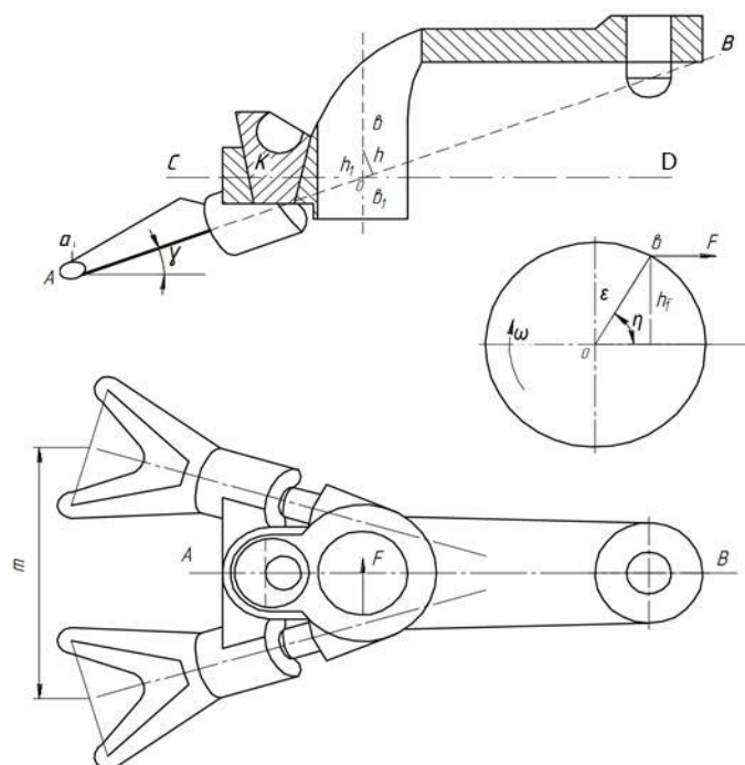
Fig. 3. Lever of the second type of clipper
