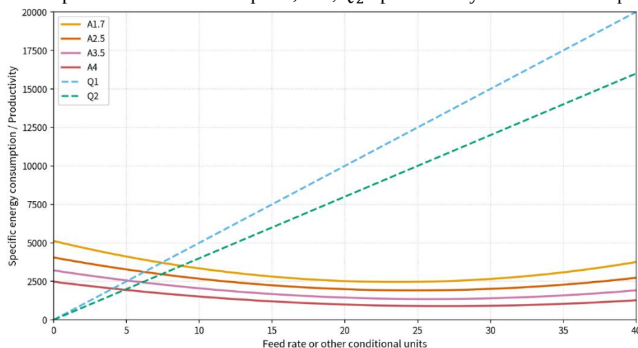
Fig. 1. Dependence of specific energy consumption and productivity of the hammer mill on drive power
