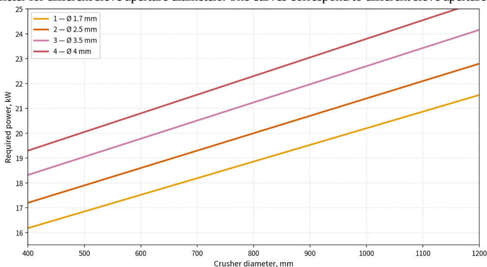
Fig. 2. Dependency of required motor power on crusher diameter
