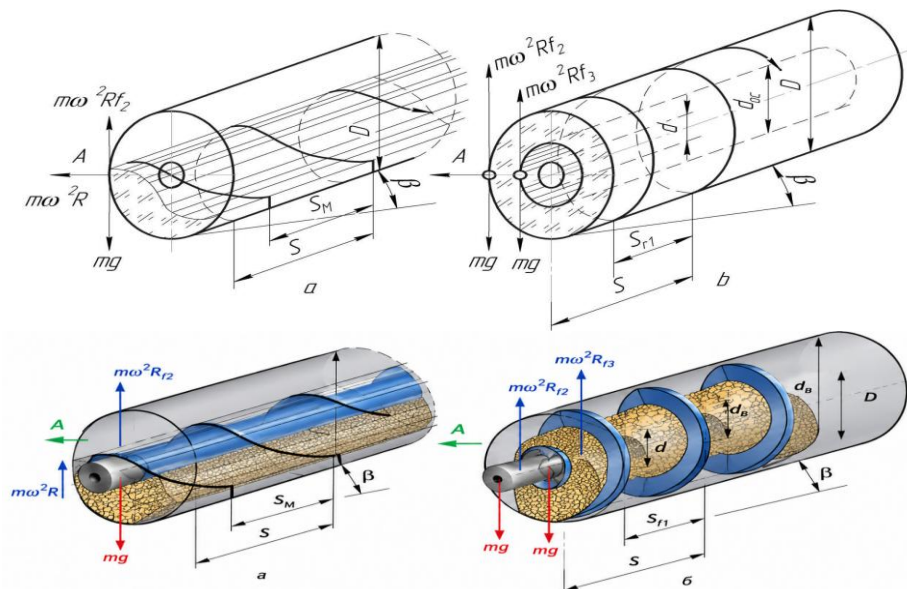
Fig. 1. Schematic diagrams of screw conveyors: (a) low-speed screw conveyor; (b) high-speed screw conveyor
