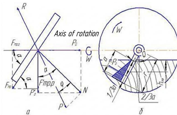
Fig. 3. Calculation schemes: (a) axial conveying velocity; (b) spiral screw
