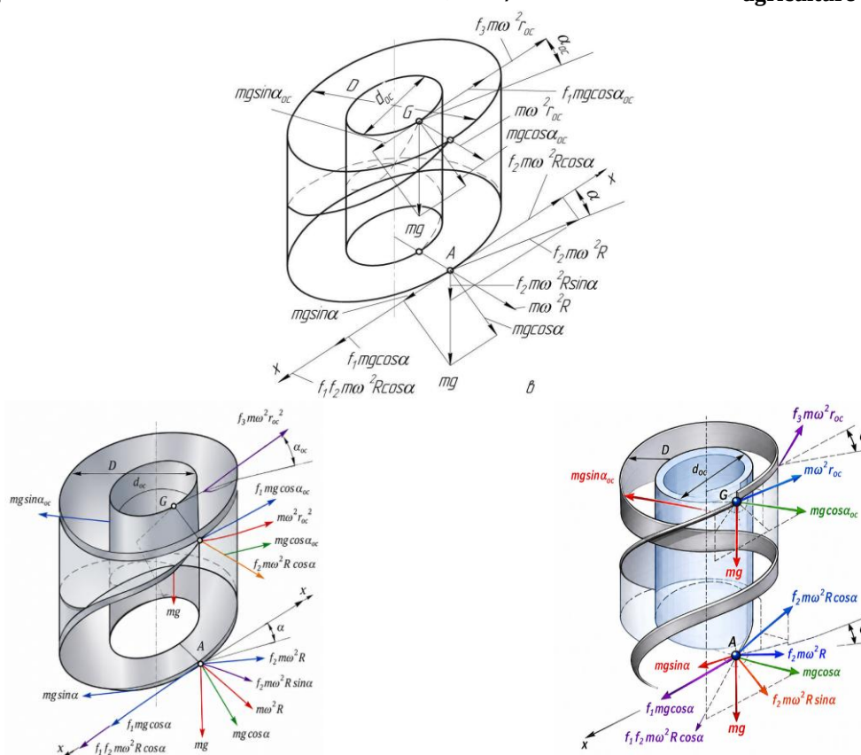
Fig. 2. Schematic diagram of a vertical screw conveyor
