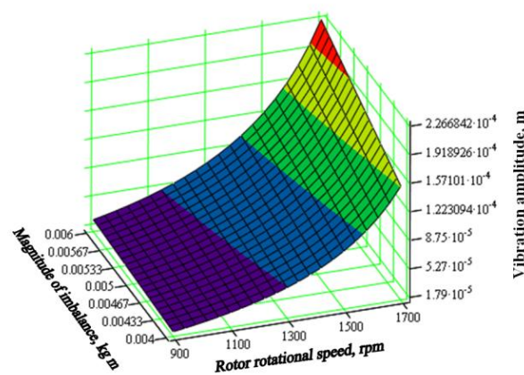
Fig. 6. Graphical dependence of the change in the rotor shaft oscillation amplitude within the range of operating frequencies
