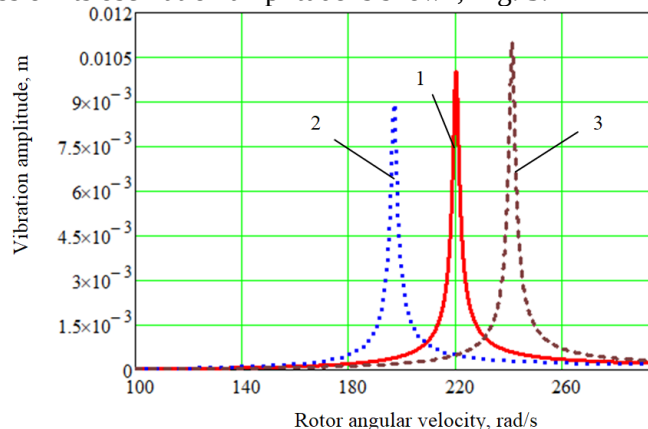
Fig. 4. Amplitude-frequency characteristic of the rotor shaft under the influence of changes in radial shaft stiffness
