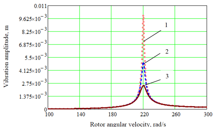
Fig. 2. Shaft oscillation amplitudes at different viscous damping coefficients
