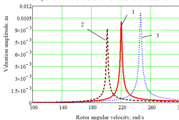
Fig. 3. Amplitude-frequency characteristic of the rotor shaft under the influence of changes in its effective mass
