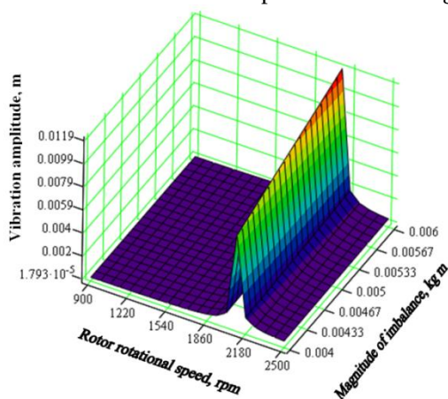
Fig. 5. Change in the rotor shaft oscillation amplitude with variation in the magnitude of imbalance
