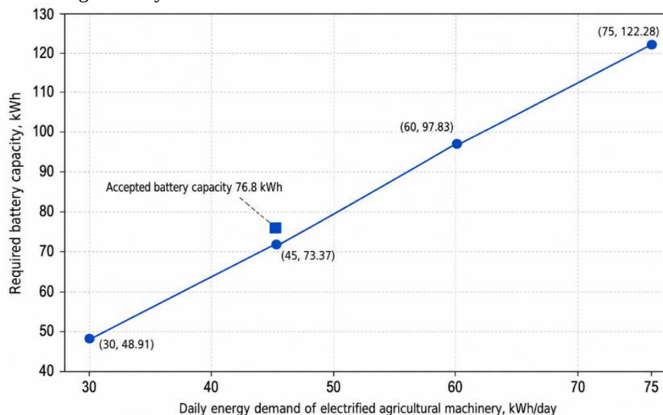
Fig. 3. Dependence of the required battery capacity on the daily energy demand of electrified agricultural machinery
