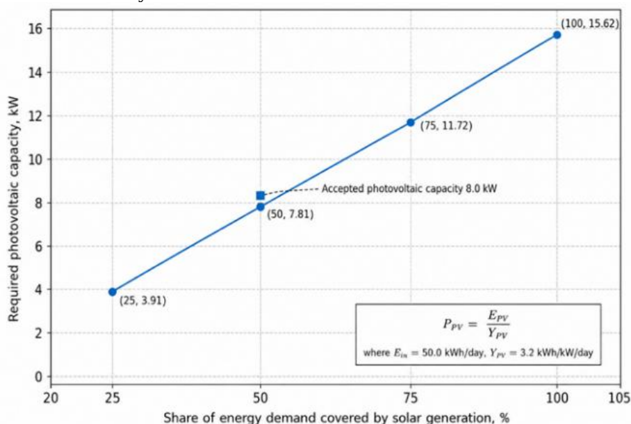
Fig. 4. Dependence of the required photovoltaic capacity on the share of energy demand covered by solar generation
