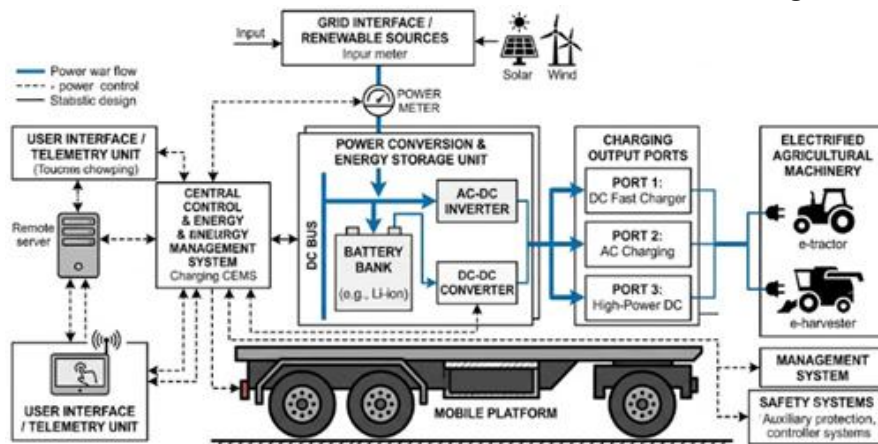
Fig. 1. General structure of a mobile charging station for electrified agricultural machinery
