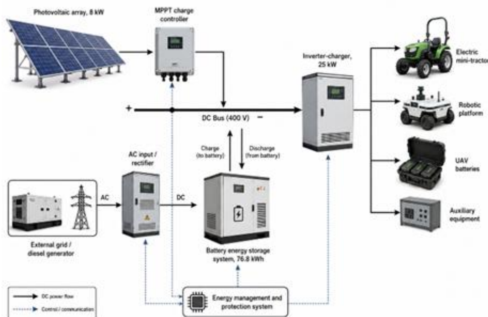
Fig. 2. Energy flow diagram of the mobile charging station
