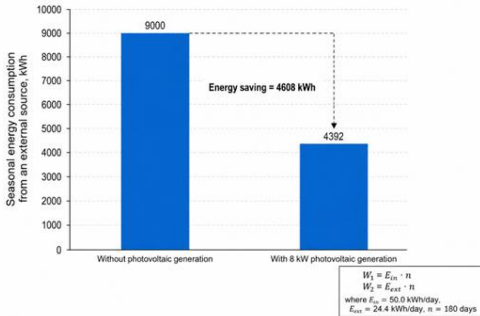
Fig. 5. Comparison of seasonal energy consumption from an external source with and without photovoltaic generation
